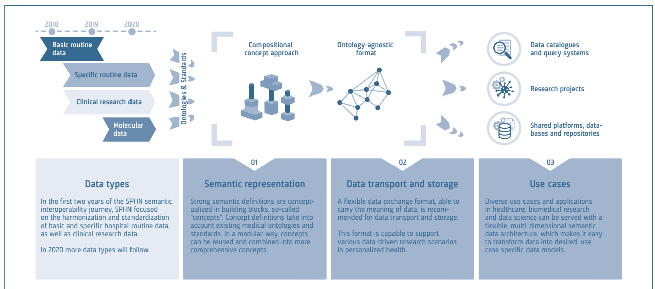
Figure 6: The SPHN Semantic Interoperability Framework.
